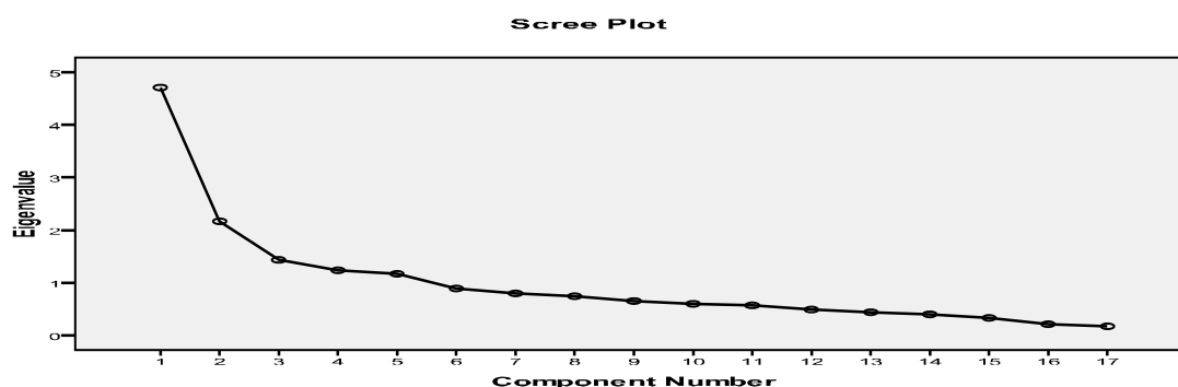
Fig. 1 Scree Plot
