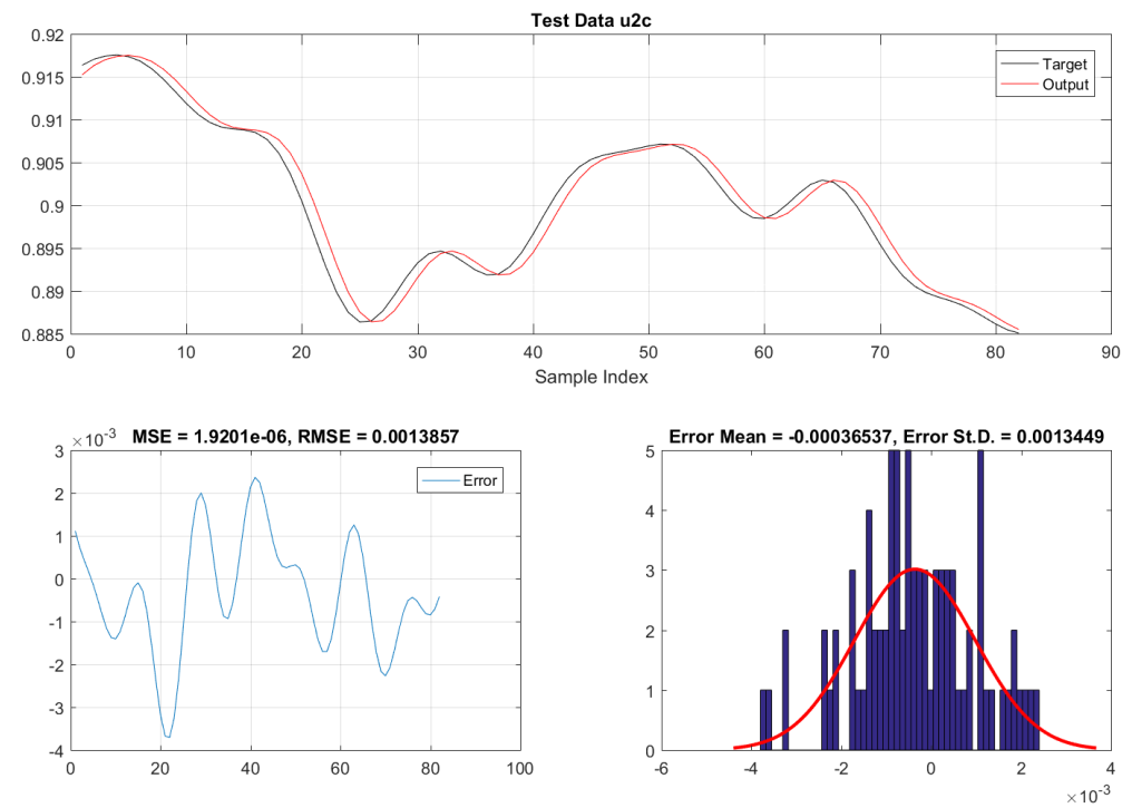
Fig. 12 Test Dataset GBP/USD with EWT
