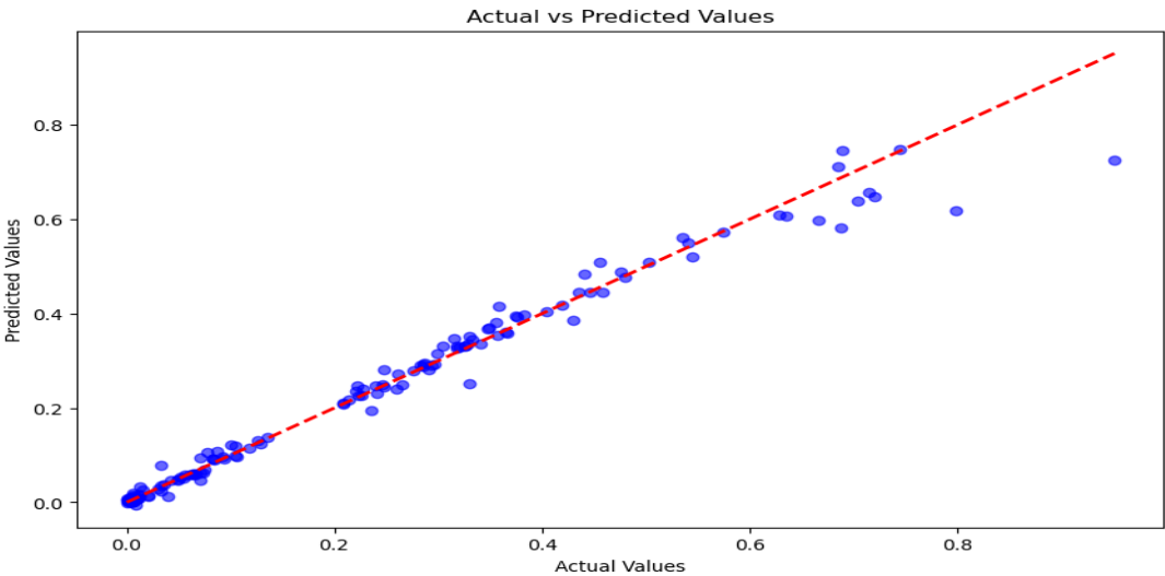
Fig. 2 Actual vs. predicted by XGBoost model
