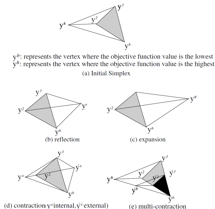
Fig. 2 Available moves in the Nelder–Mead simplex method, in the case of 3 variables
